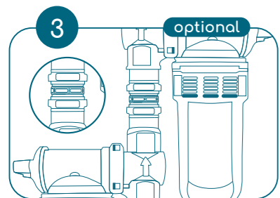
Optional - If you have a duo kit: connect both devices with the spacer (C)
