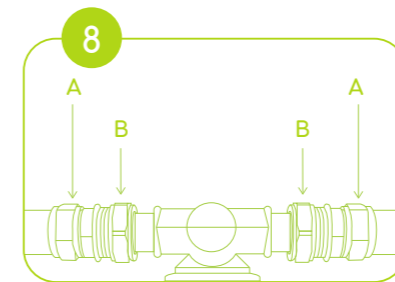
Connect connectors (A) to couplings (B)* and fix the connectors (A) firmly
